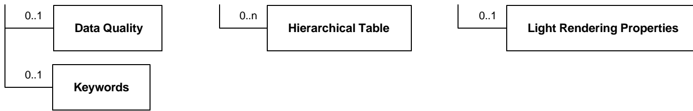
Diagram 6.9--DRM_Alternate_Hierarchy_Related_Geometry
