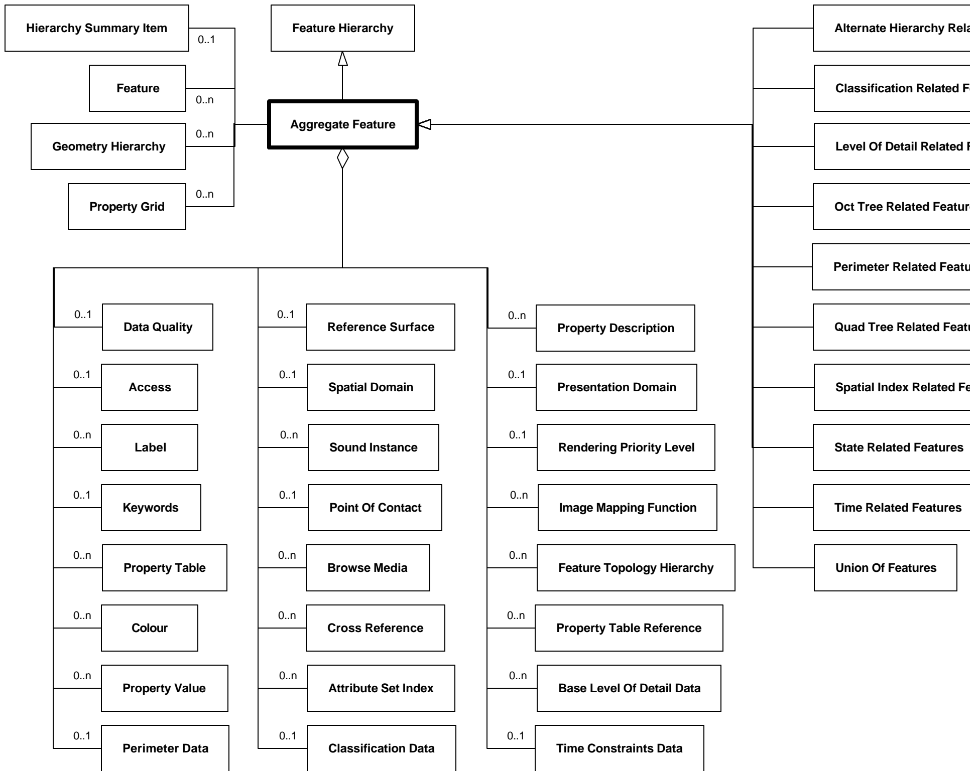
Diagram 6.5--DRM_Aggregate_Feature
