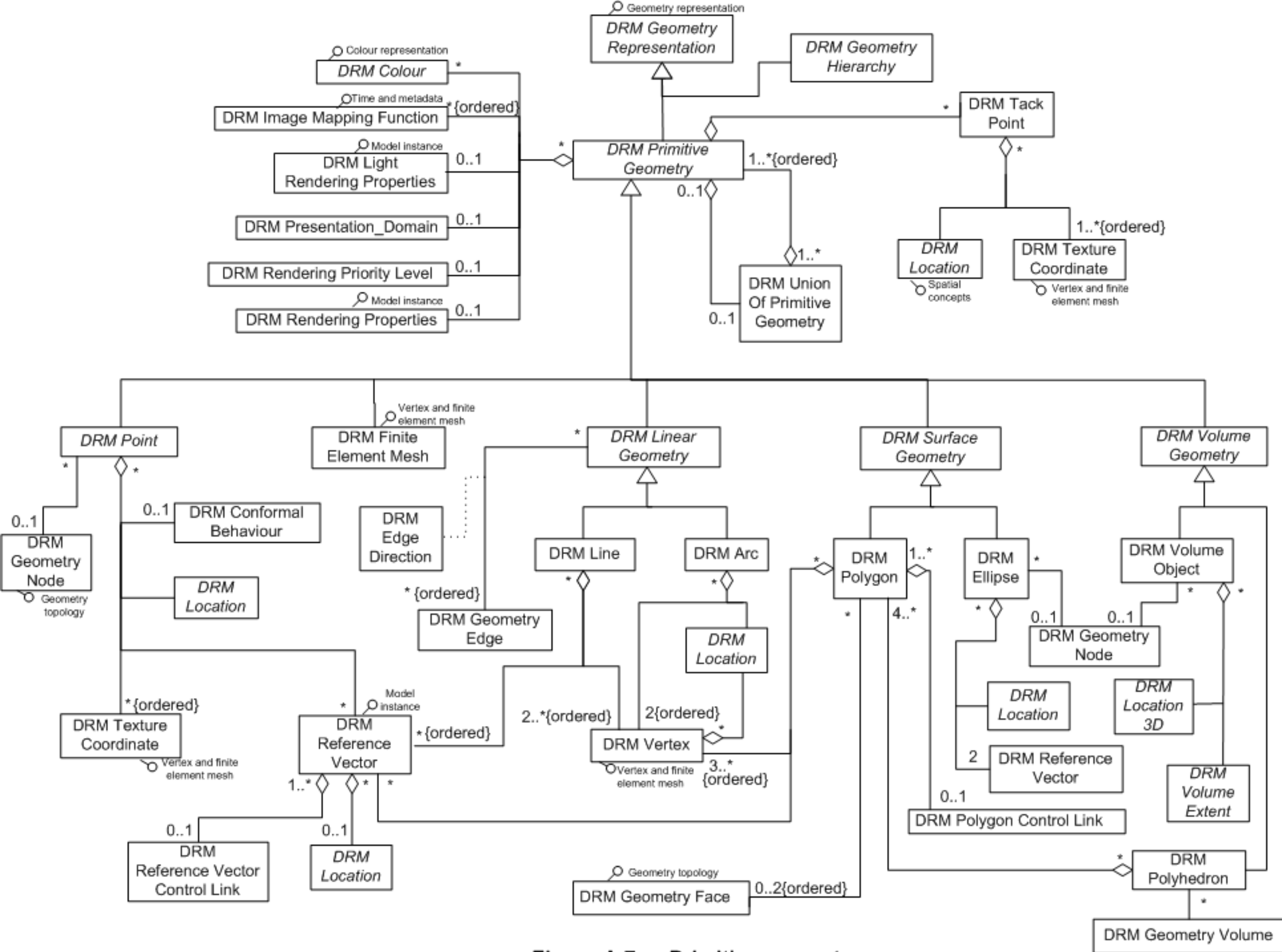
Figure A.7 — Primitive geometry
