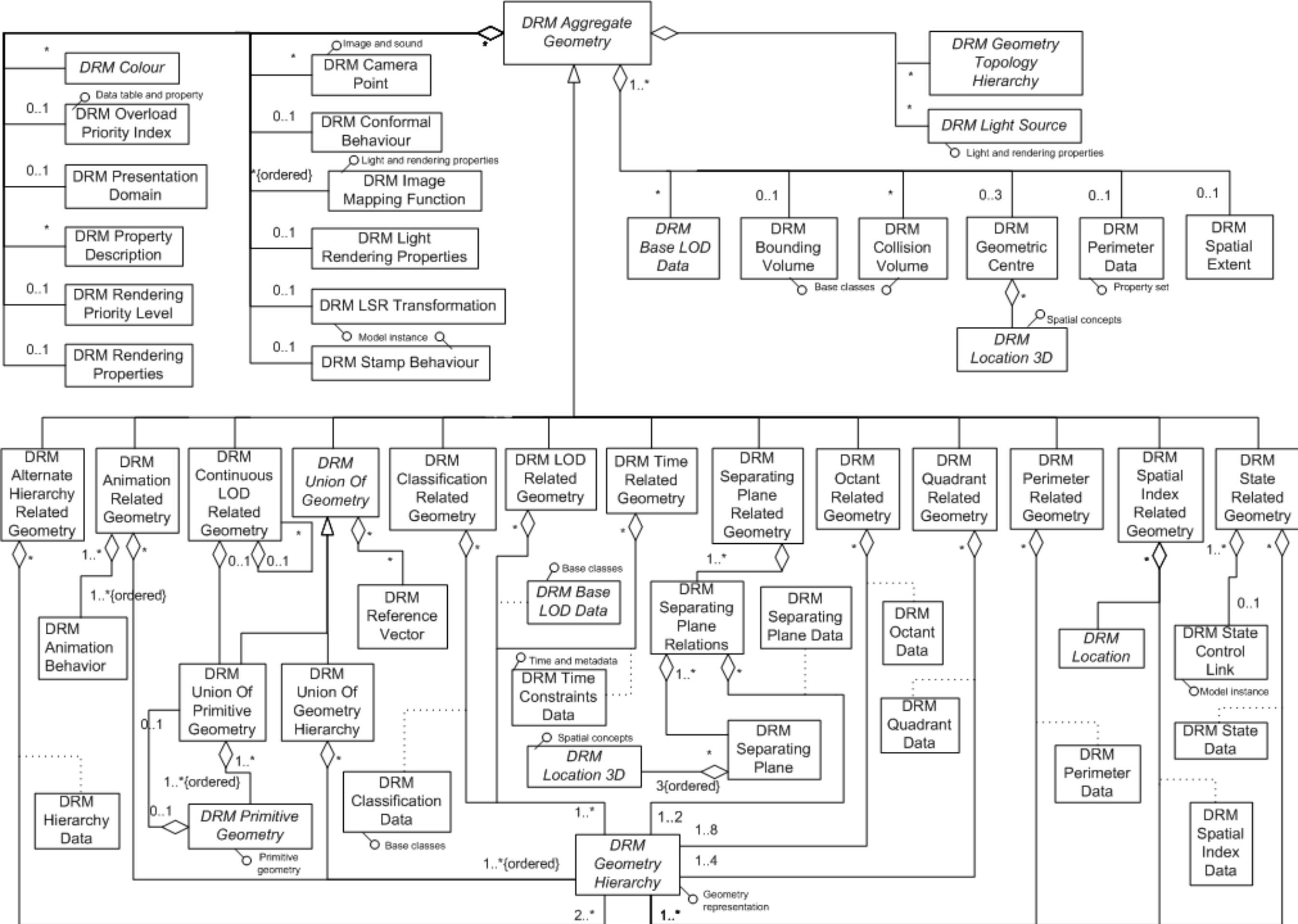
Figure A.6 — Aggregate geometry
